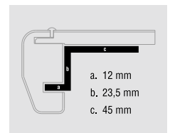
An alternative solution aluminium anodised stair nose profiles to cover stair treads
