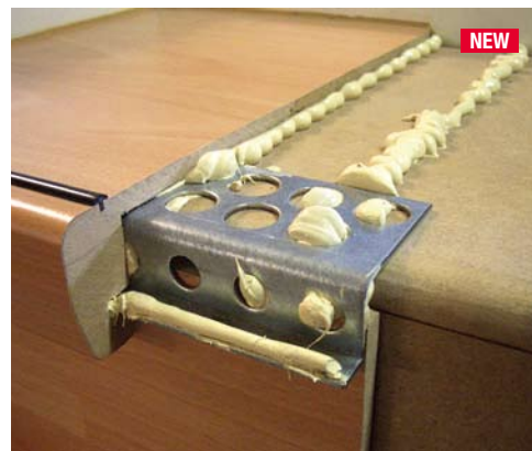
Stabilising profile to level and stabilise the tread
